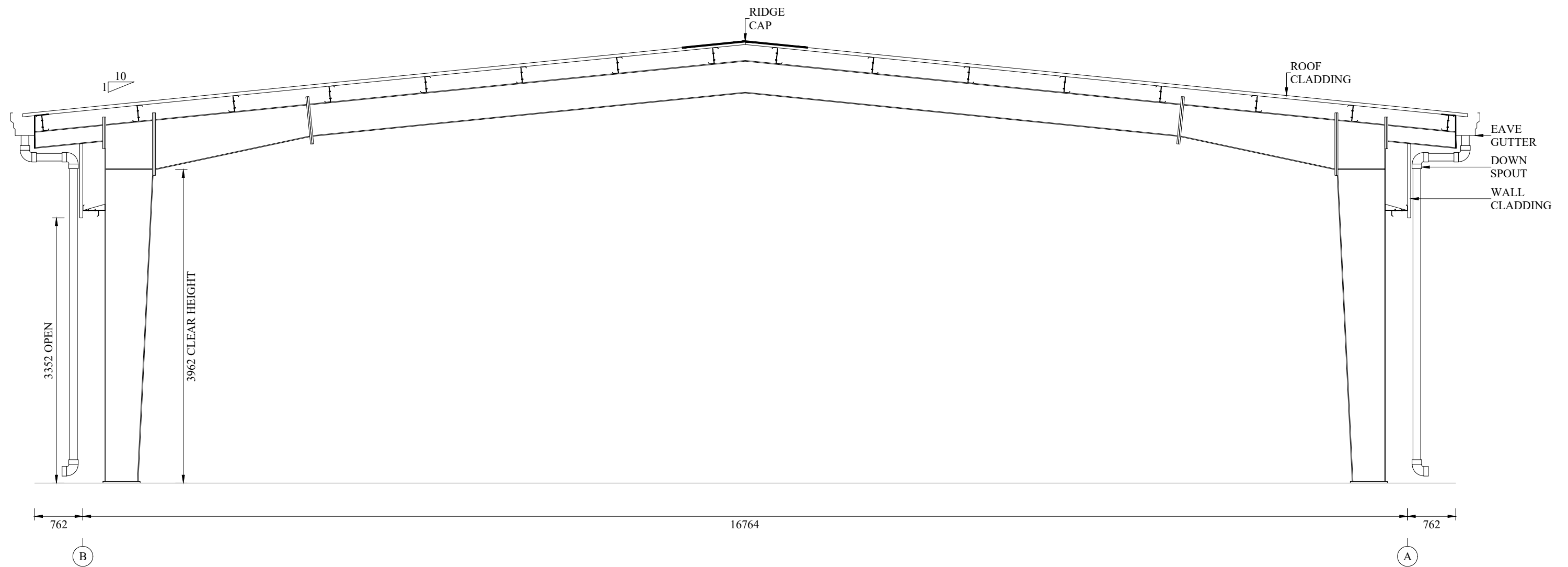
CROSS SECTION GRID @ 1 to 13
