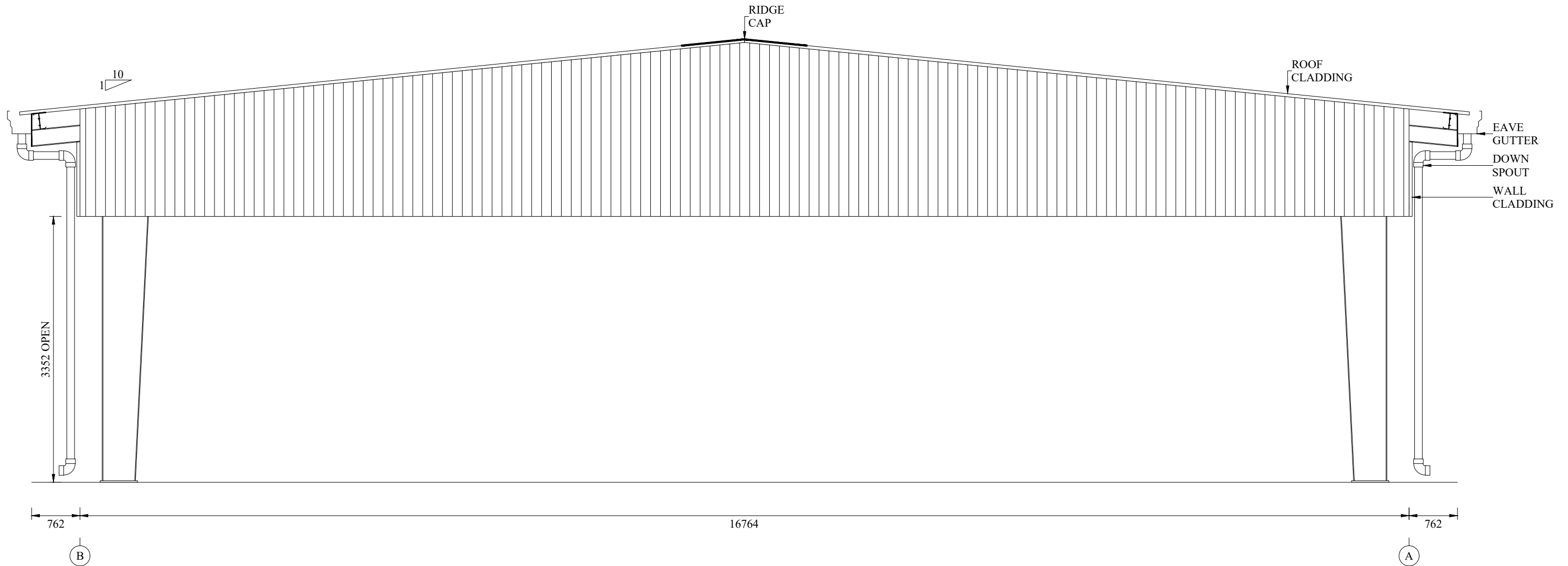
END WALL ELEVATION GRID @ 1
