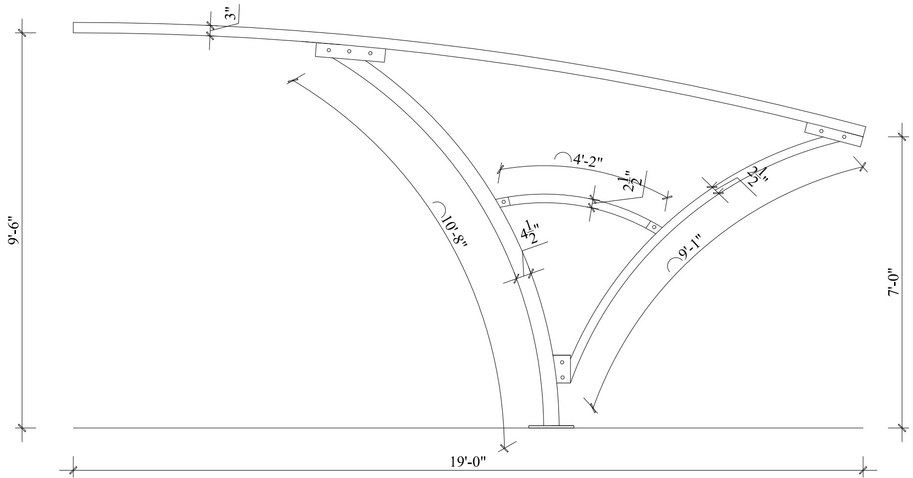
SINGLE PARKING SHADE
