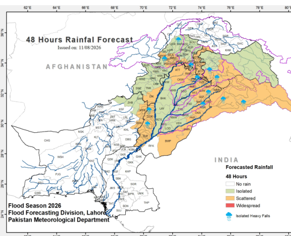
Rainfall outlook — next 48 hours
