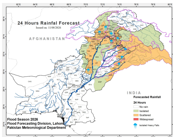
Rainfall forecast — next 24 hours
