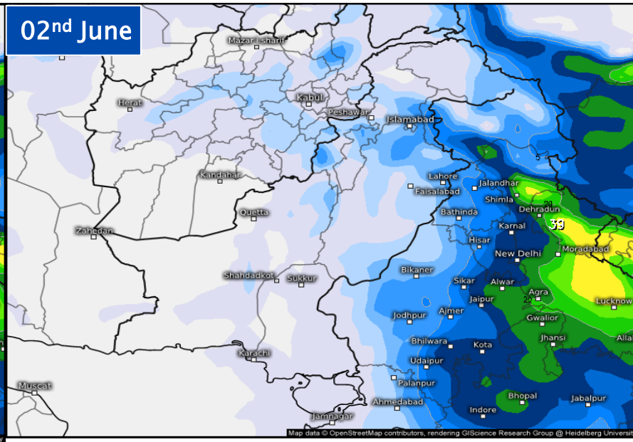
Accumulated total precipitation (mm) From Wed 05/27/2026, 07:00pm CDT to Tue 06/02/2026, 01:00am CDT
