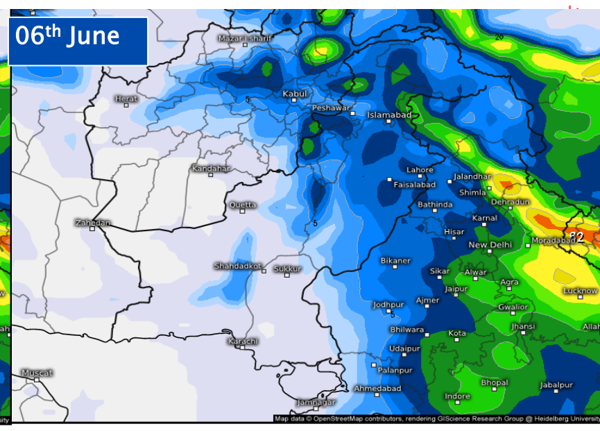
Accumulated total precipitation (mm) From Wed 05/27/2026, 07:00pm CDT to Sat 06/06/2026, 01:00pm CDT
