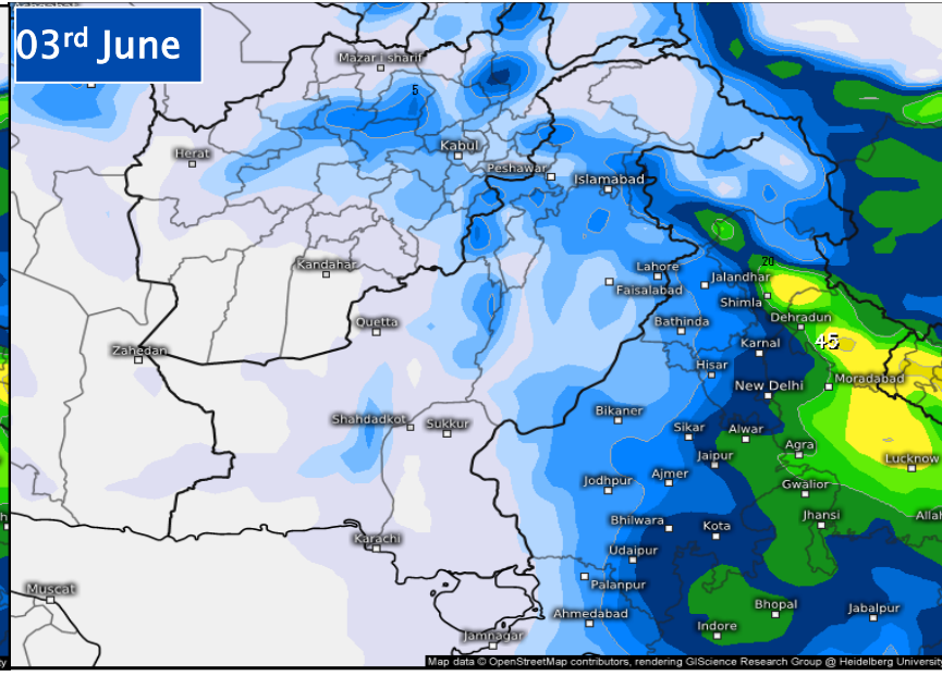
Accumulated total precipitation (mm) From Wed 05/27/2026, 07:00pm CDT to Wed 06/03/2026, 07:00am CDT
