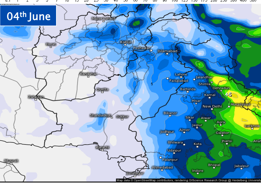
Accumulated total precipitation (mm) From Wed 05/27/2026, 07:00pm CDT to Thu 06/04/2026, 01:00am CDT
