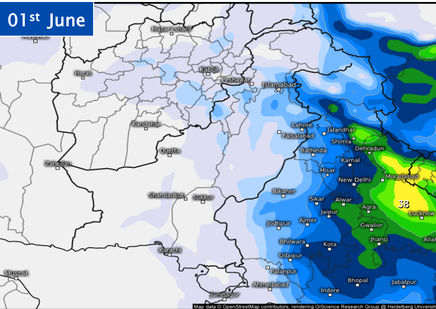
Accumulated total precipitation (mm) From Wed 05/27/2026, 07:00pm CDT to Mon 06/01/2026, 01:00am CDT
