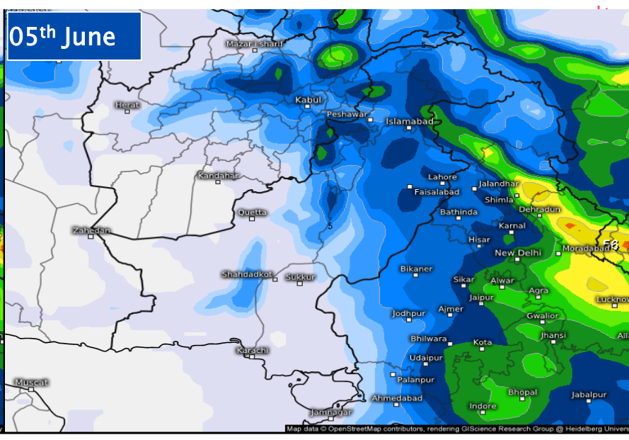
Accumulated total precipitation (mm) From Wed 05/27/2026, 07:00pm CDT to Fri 06/05/2026, 01:00pm CDT
